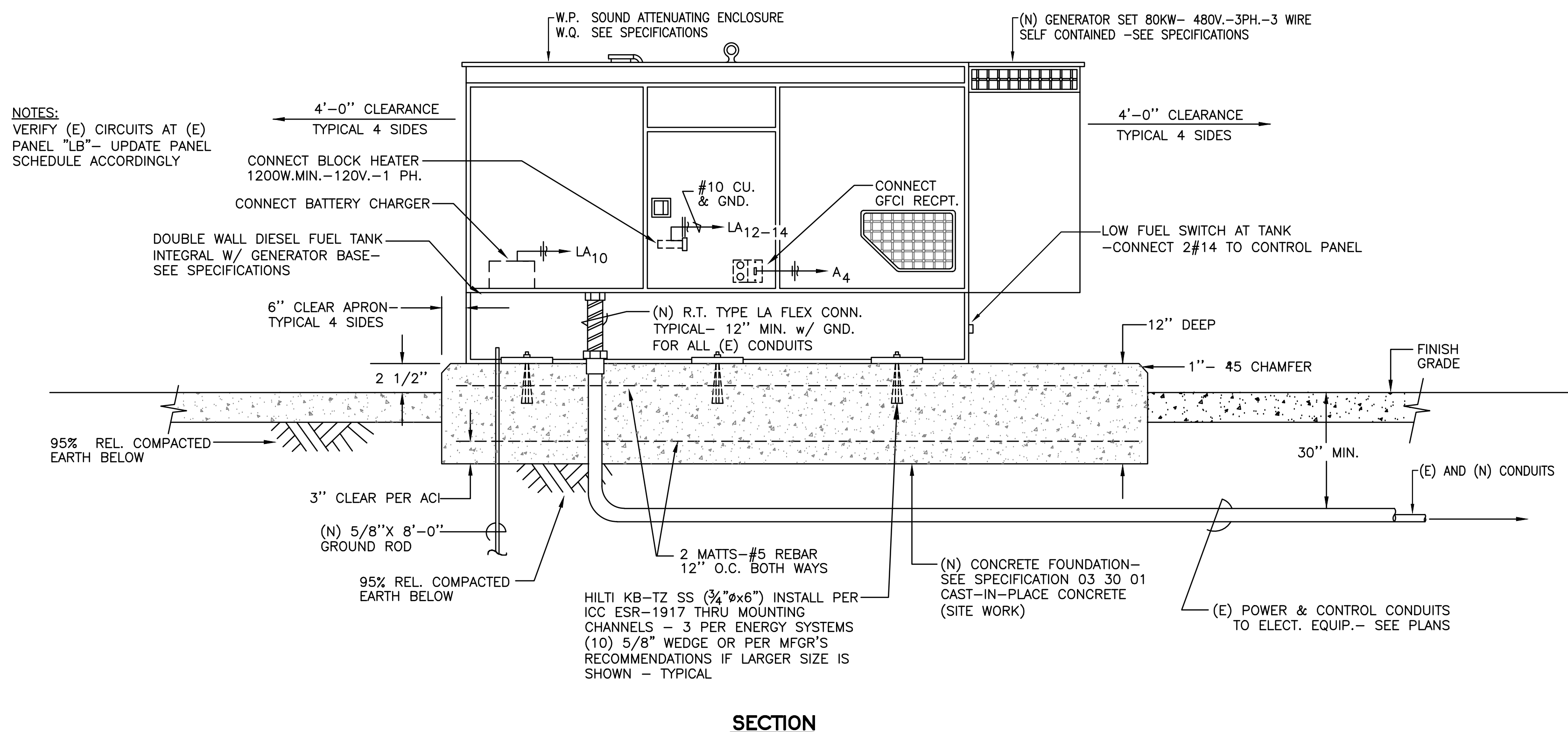
5 NEW GEN-SET AND FOUNDATION SCALE: NTS
