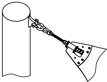
Fabric Connection
