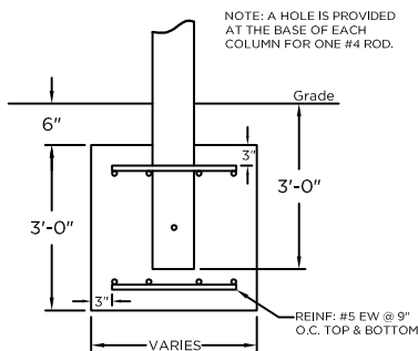
Footer Detail
