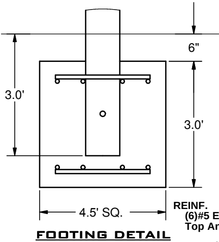
FOOTING DETAIL
