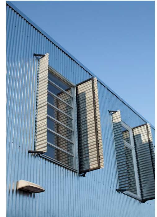
+ Vertical fin sun shade for east and west-facing windows
