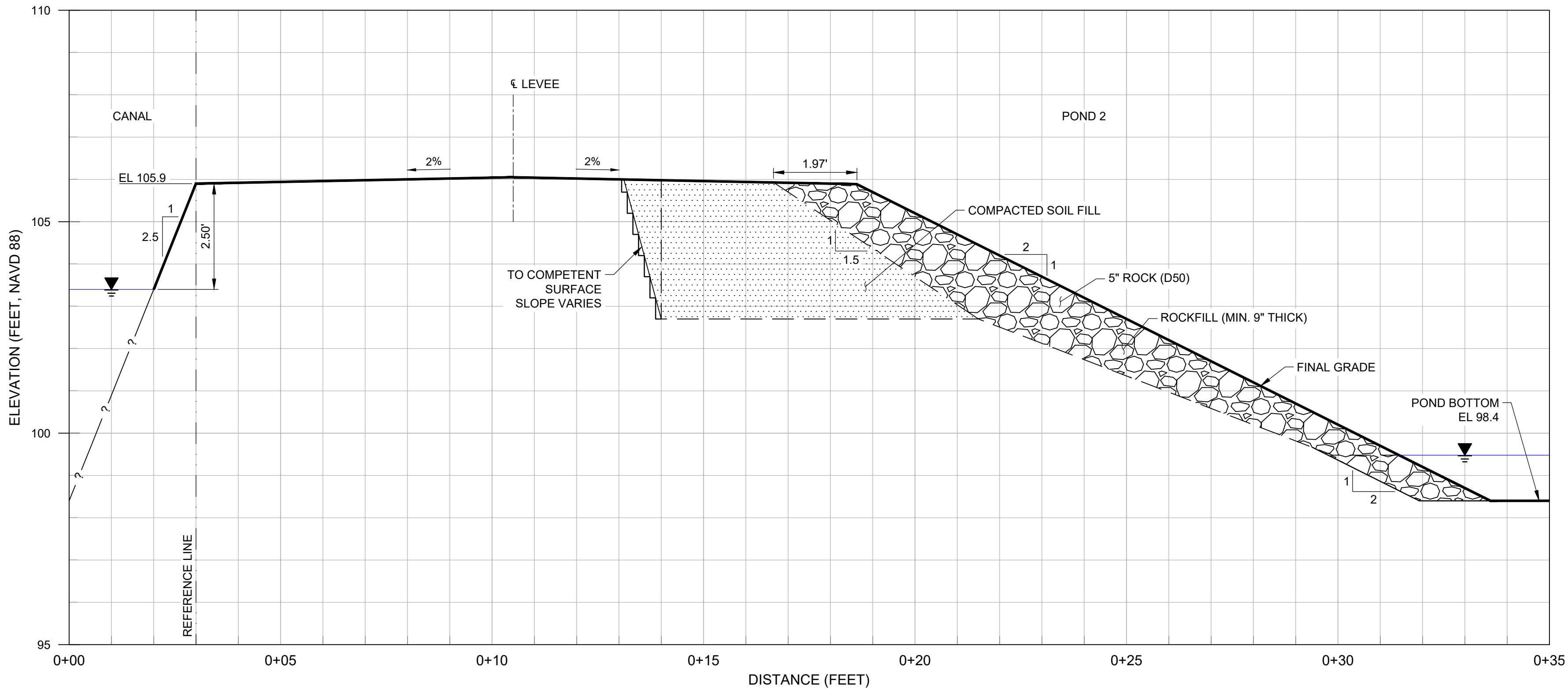
TYPICAL SECTION - REACH 2 - STA 210+50 TO STA 219+40
