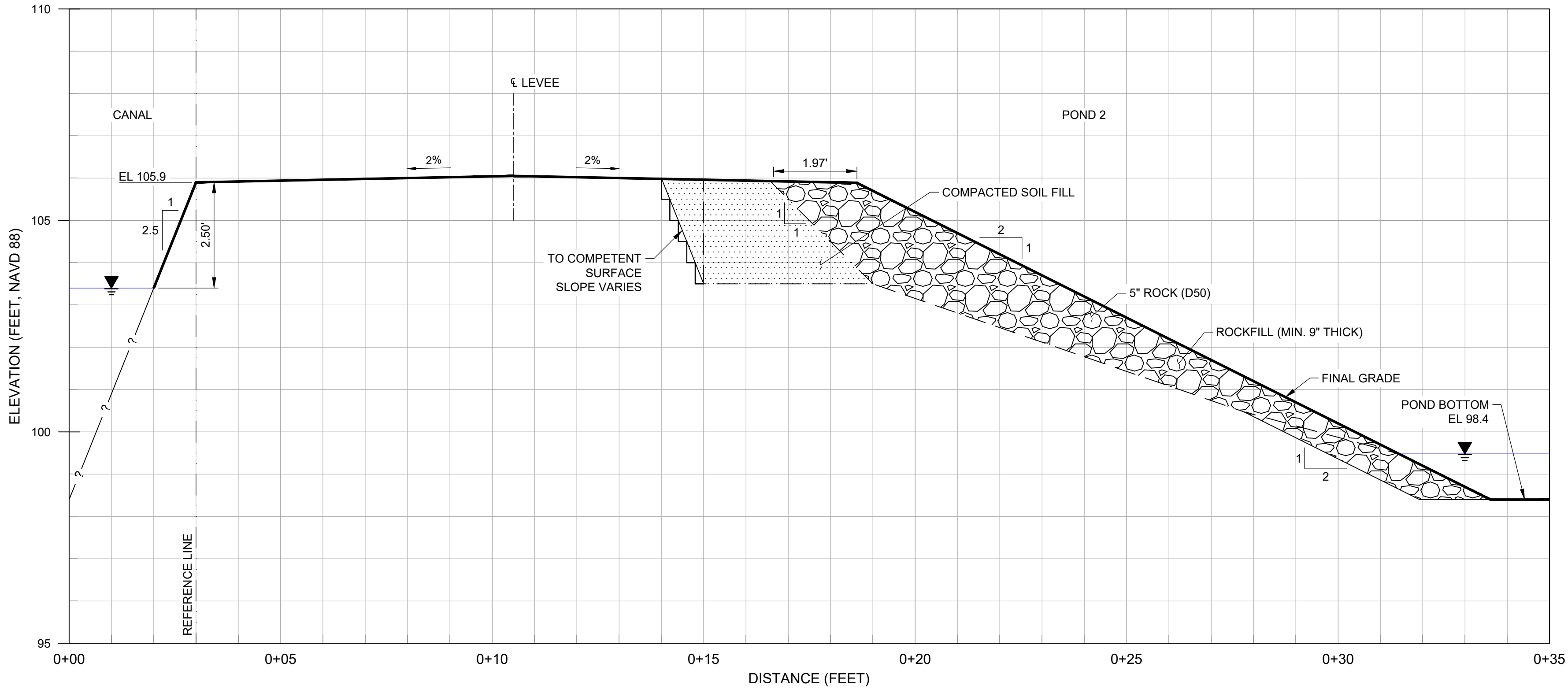
TYPICAL SECTION - REACH 1 - STA 205+00 TO STA 210+50
